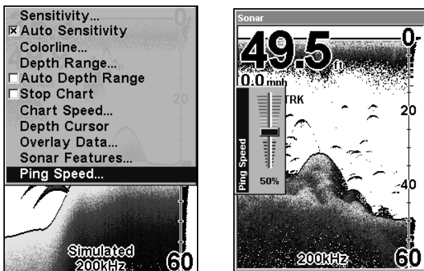
Sonar Menu (left) with Ping Speed command selected. Ping Speed Control Bar (right) at default setting.
